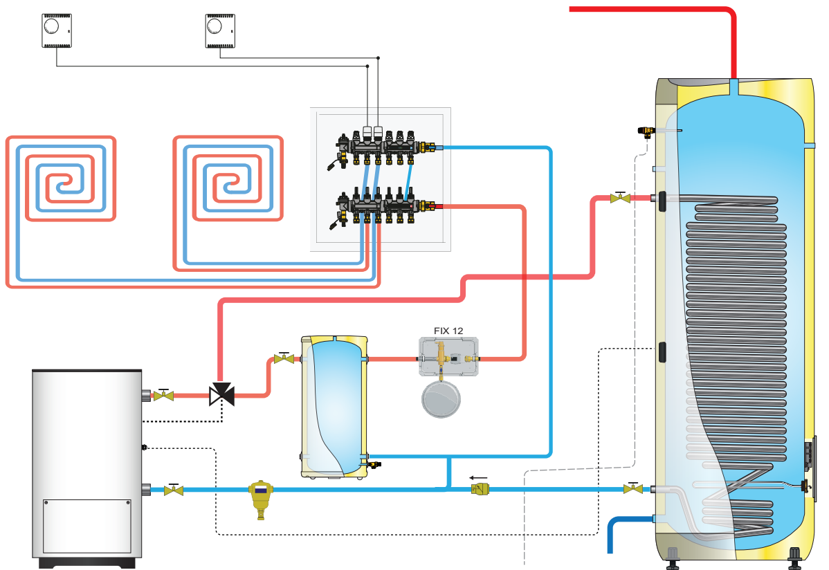
Delta Geocoil DGC 300
